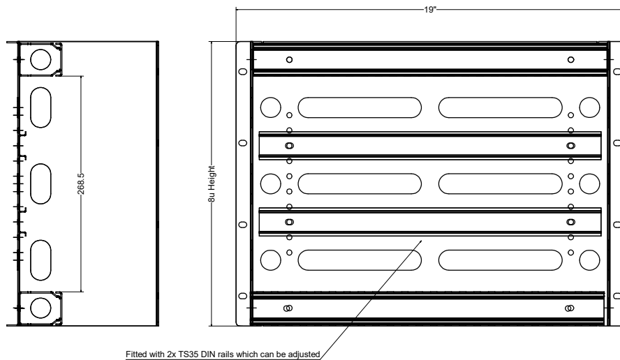
Fitted with 2x TS35 DIN rails which can be adjusted
