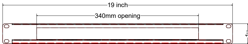
Cable lacing panel raised to keep cables straight
